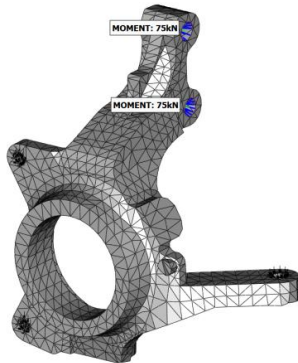
Figure 4: Loading conditions on initial mesh
