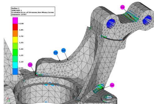
Figure 8: Probable error after first refinement
