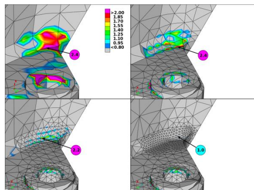
Figure 9: Probable error values are minimized after four iterations
