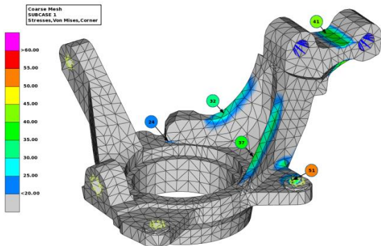
Figure 5: Von Mises Stress results at first iteration
