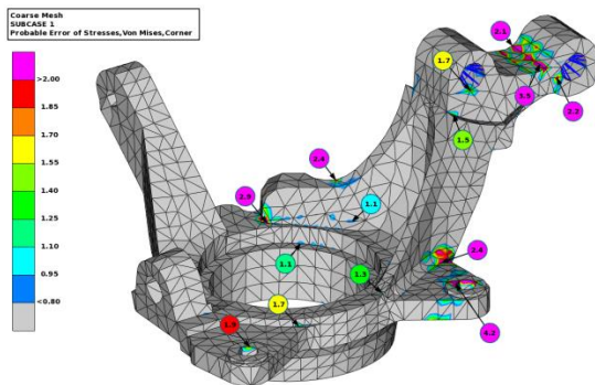
Figure 6: Areas where the probable error is more than 1 at first iteration
